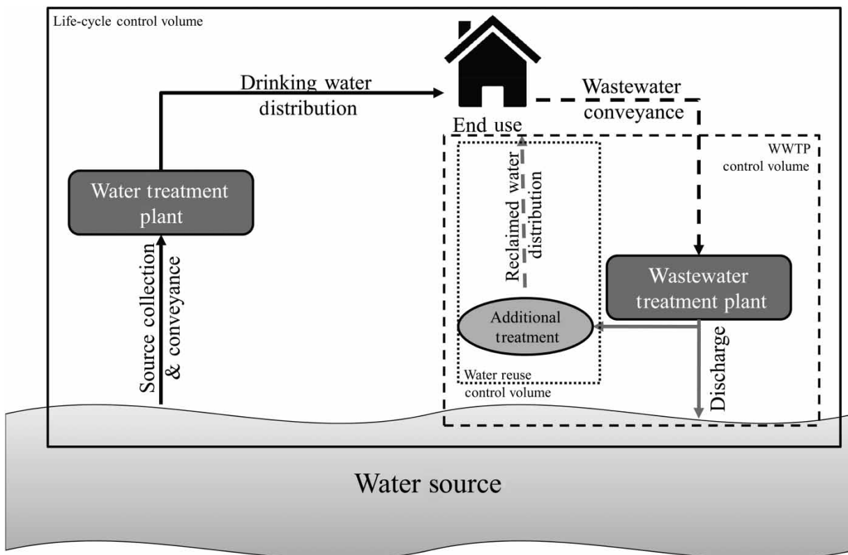
Figure 2 | Accounting for energy use for reclaimed water depends on how the control volume boundary is drawn. When considering the life-cycle control volume (solid line), energy use includes that associated with drinking water, wastewater treatment, and reclaimed water distribution. The wastewater treatment plant (WWTP) control volume (dashed line) includes energy consumption for wastewater treatment and reclaimed water distribution. The water reuse control volume (dotted line) includes only additional treatment (if necessary) and reclaimed water distribution.
